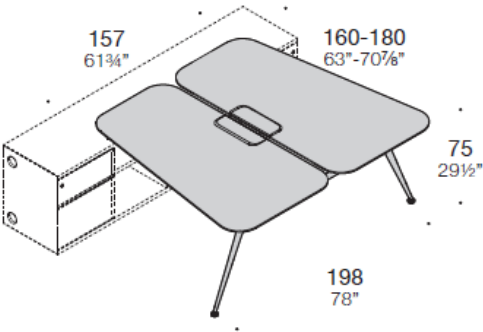
Trapezoid top for bench with pivot top access and cable trays
