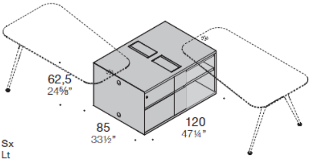
W120 (47¼ ") D85 (33½ ") two-faces base with 2 open cabinets + 2 drawers and 2 drawer cabinets
