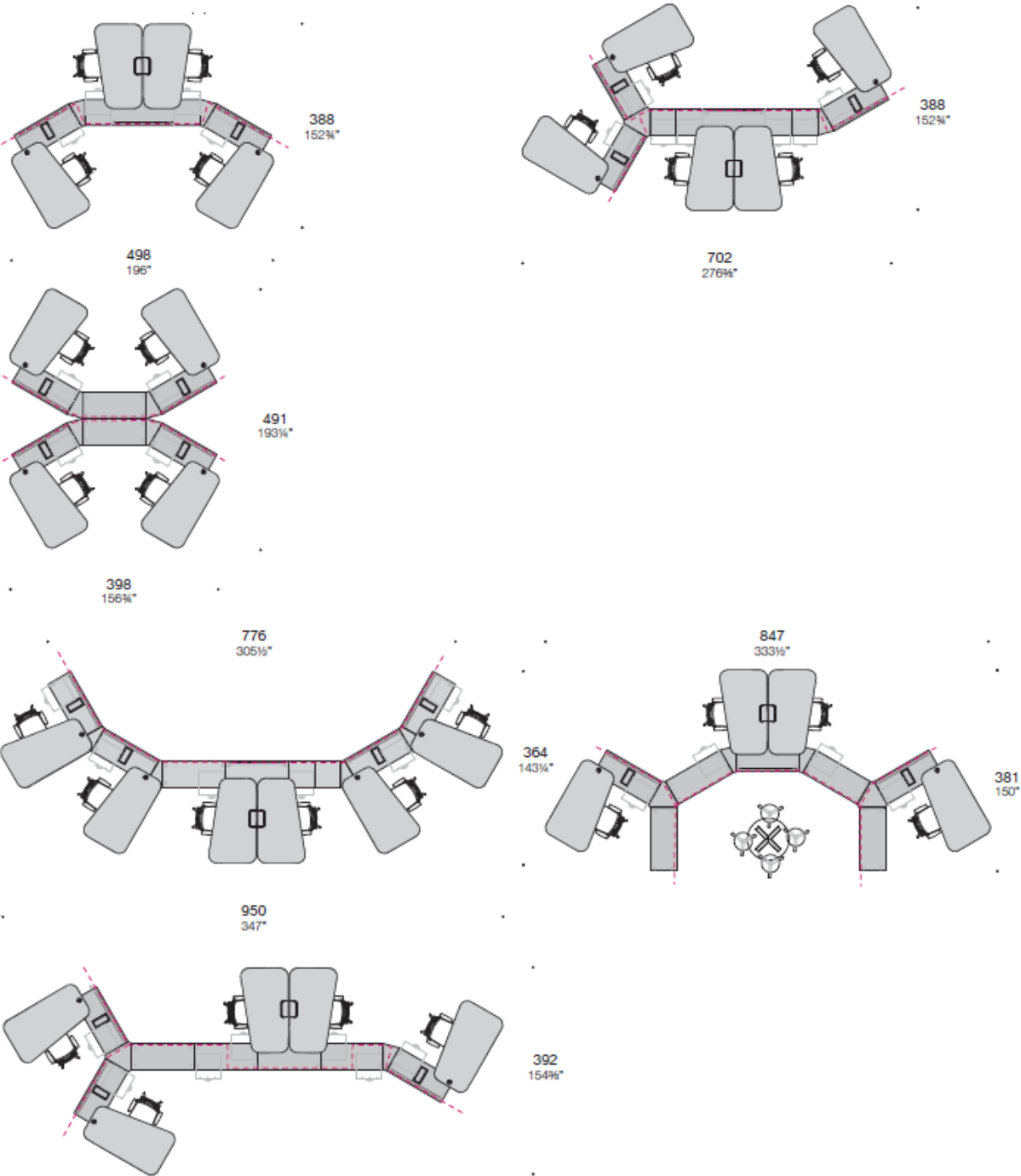
Frattale with D50 (19 1/8 ") bases
