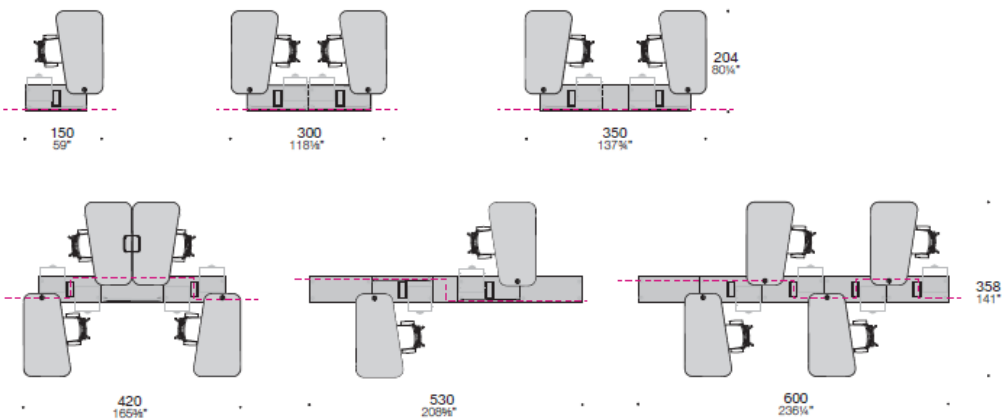
Cartesio with D50 (19 5/8") bases
