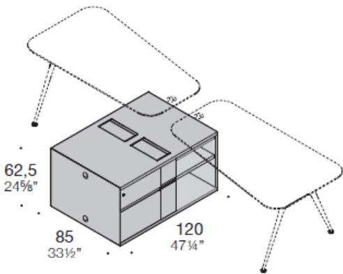
W120 (47¼ ") D85 (33½ ") two-faces base with 2 open cabinets + 2 drawers and 2 drawer cabinets
