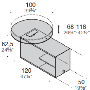
W120 (47 1/4 ") base with rounded sit&stand top
