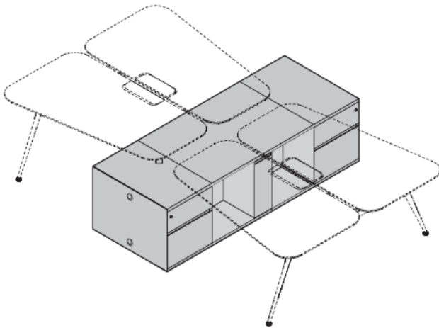
W220 (86 5/8 ") P85 (33 1/2 ") two-faces base with 4 drawers and 4 drawer cabinets
