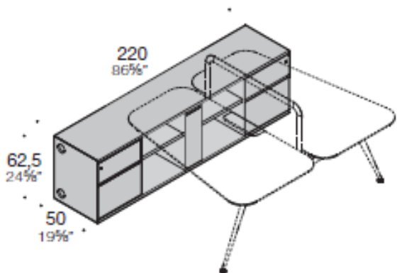
W120 (47 1/4 ") D50 (19 5/8 ") base for 2 seater bench
