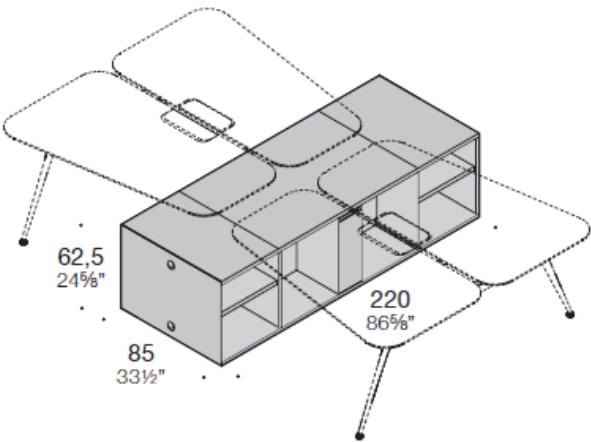
W220 (86 5/8 ") P85 (33 1/2 ") two-faces base with open front compartment
