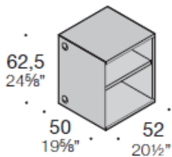
W52 (20½ ") side base with open front compartment
