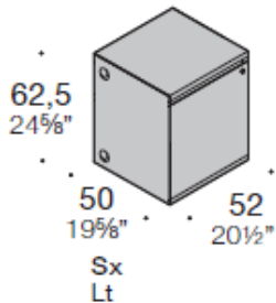
W52 (20½ ") side base with hinged door
